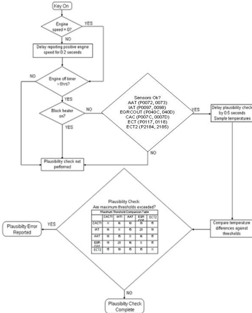
Figure : Air Temperature Plausibility Check Flow Chart
